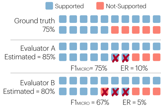
Figure 3: A case in which F1_{\text{MICRO}} and Error Rate (ER) rank two evaluators differently. Evaluator A is better in F1_{\text{MICRO}} , and Evaluator B is better in ER.
